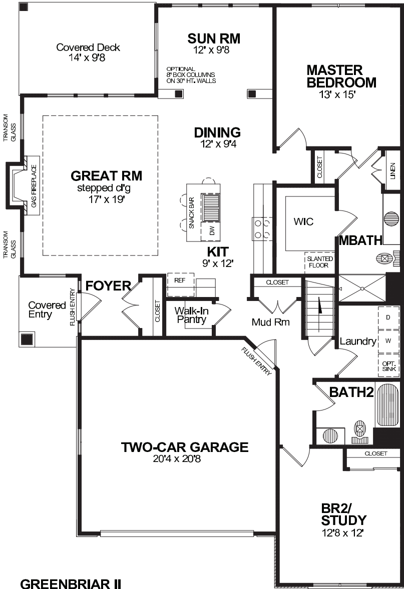
GREENBRIAR II MAIN FLOOR 1624 SF
